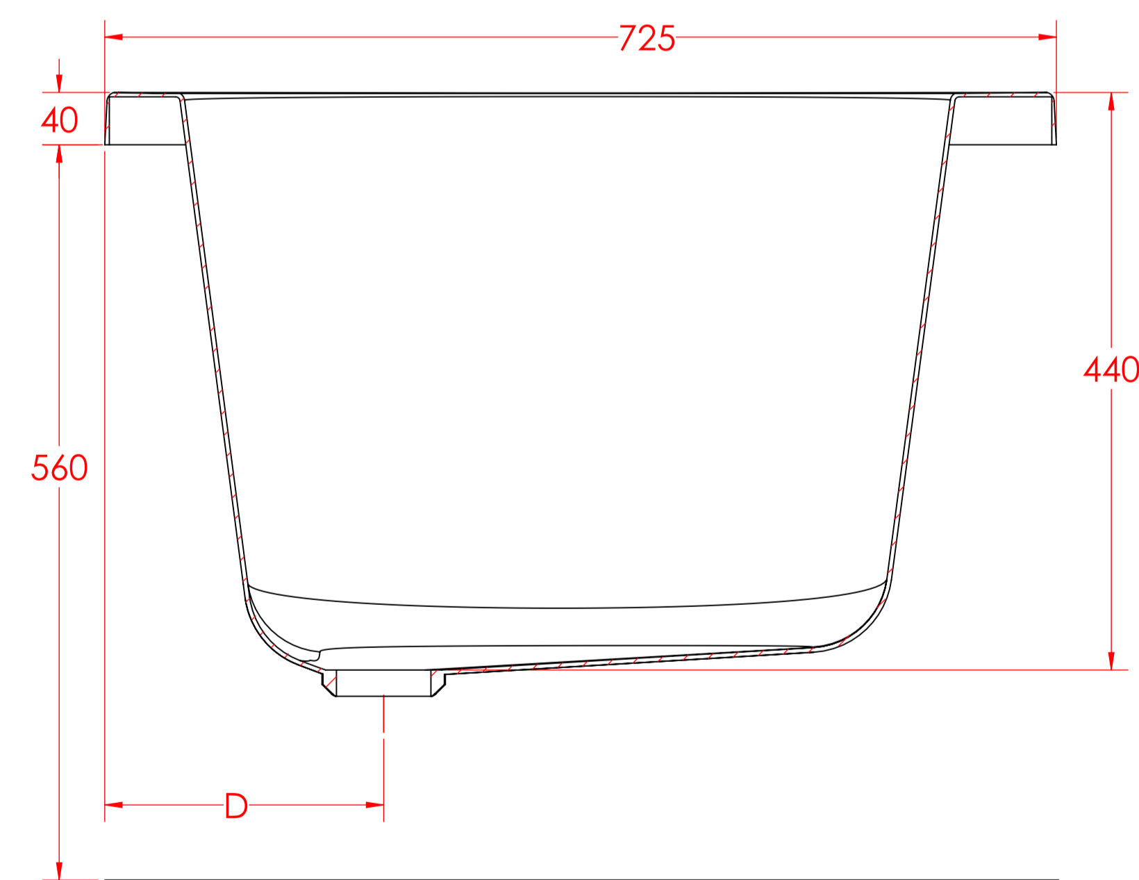
SECTION E-E SCALE 1 : 4
