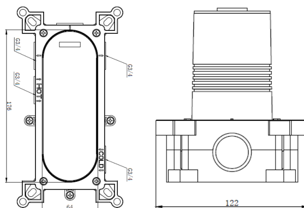
Dimensions (measurements in mm)
